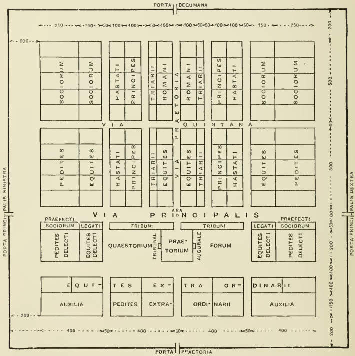
PLAN OF ROMAN CAMP,
